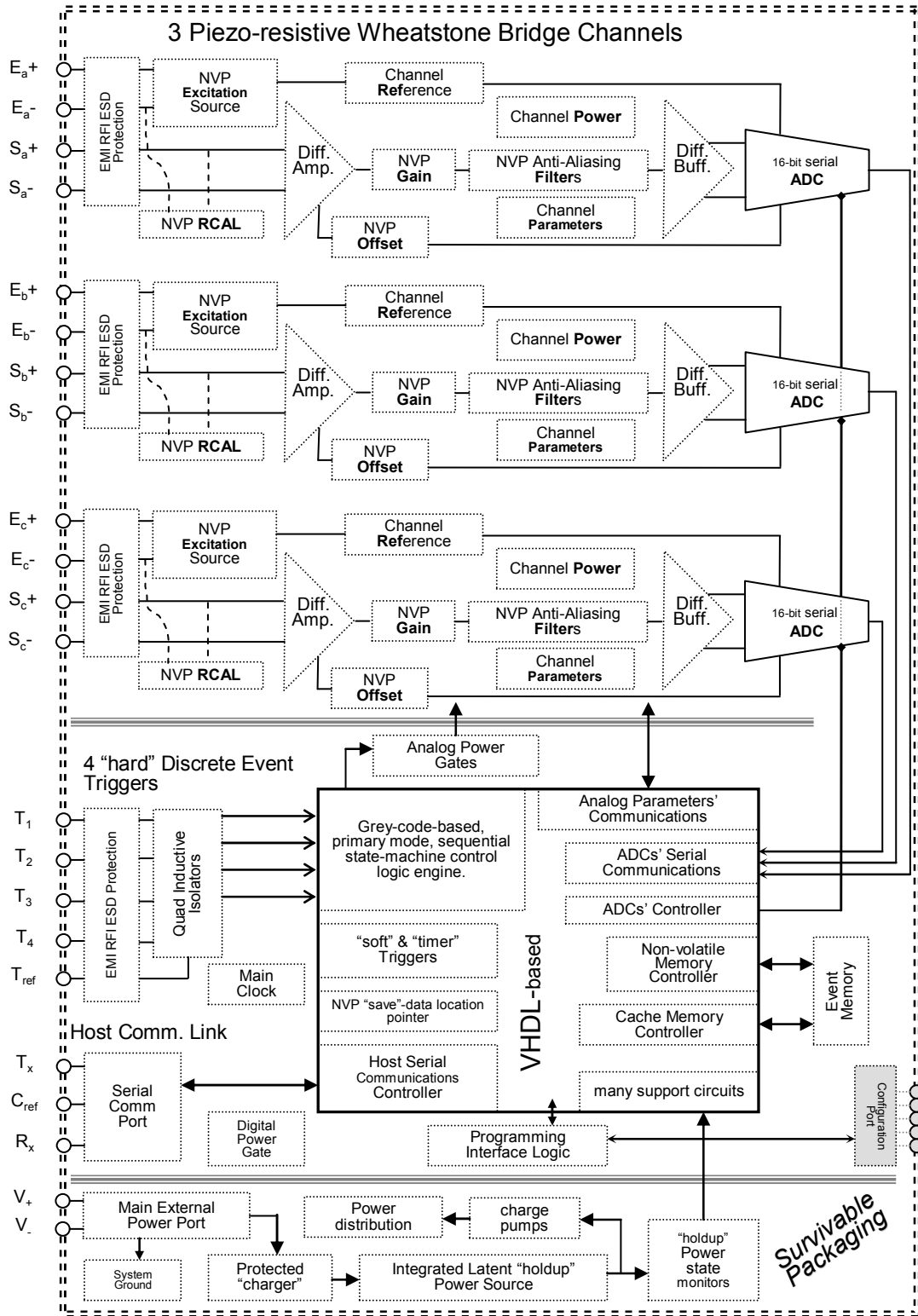
Figure 1: SER's Functional top-level Block Diagram
